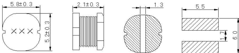
Land Pattern
