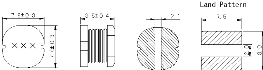
Land Pattern
